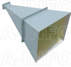
LB-430-20-A Standard Gain Horn Antenna 1.7-2.6GHz 20dB Gain Rectangular Waveguide Interface
